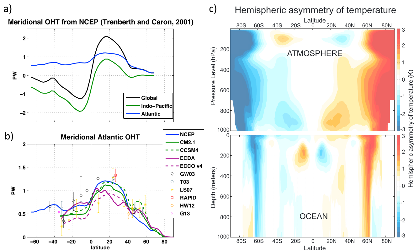
Figure 3. (a) Meridional ocean heat transports (OHT, positive northward) in PW (10 15 W) for the global ocean (black), the Indo-Pacific (green), and the Atlantic (blue) from NCEP atmospheric reanalysis [Trenberth and Caron, 2001]. (b) Atlantic OHT from NCEP atmospheric reanalysis (blue) [Trenberth and Caron, 2001] is compared to several direct estimates: Ganachaud and Wunsch [2003] (black diamonds), Talley [2003] (grey circles), Lumpkin and Speer [2007] (yellow stars), the RAPID-MOCHA array at 26.5°N (red square) [Johns et al., 2011], Hobbs and Willis [2012] (orange diamond), and Garzoli et al. [2013] (magenta cross). The vertical bars indicate the uncertainty range for the direct estimates. Also compared are the Atlantic OHT in CM2.1 (green solid) and CCSM4 (green dashed) preindustrial control simulations (modified from Msadek et al. [2013]) and the GFDL ECDA (1960–2010, solid purple) [Chang et al., 2012] and ECCO v4 (1992–2012, dashed purple) [Forget and Ponte, 2015; Forget et al., 2015] ocean state estimates. (c) Observed hemispheric asymmetry of temperature in the atmosphere and ocean (in °C) computed from the NCEP reanalysis and the World Ocean Atlas. The asymmetric component of a temperature field T(\phi) is defined as T_{as}(\phi) = (T(\phi) - T(-\phi))/2 where \phi is the latitude [from Marshall et al., 2014a].
