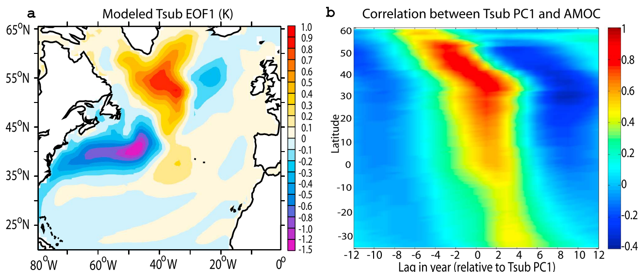
Figure 10. (a) First empirical orthogonal function (EOF1) of temperature at 400 m ( T_{\text{sub}} ) (K, 24.8% of variance) from a 1000 year control run of GFDL CM2.1 [from Zhang, 2008]. (b) Correlation between the first principle component (PC1) time series of T_{\text{sub}} and AMOC strength variations at all latitudes. The AMOC strength at each latitude is defined as the maximum of the annual mean zonally integrated Atlantic overturning stream function in density space [from Zhang, 2010a].
