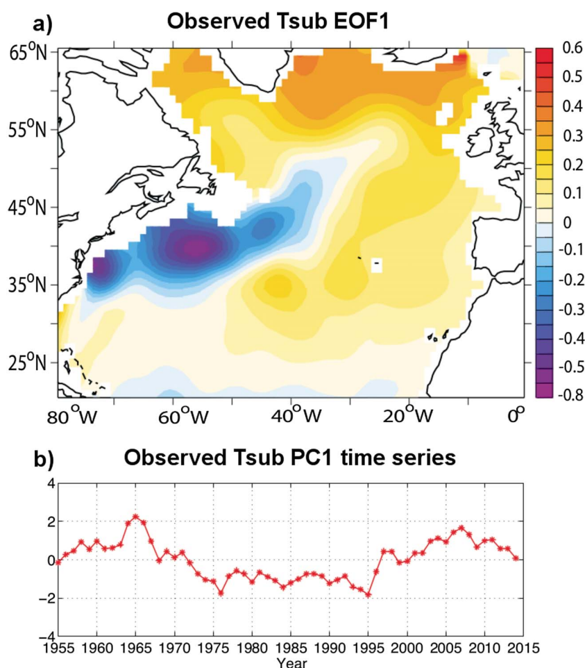
Figure 11. Variability of observed annual mean anomalies of ocean temperature at 400 m ( T_{\text{sub}} ) from an objectively analyzed ocean temperature data set [Levitus et al. , 2005]. (a) The first empirical orthogonal function (EOF1) of observed North Atlantic T_{\text{sub}} (K, 30%) for 1955–2014. (b) First principle component (PC1) time series of observed T_{\text{sub}} during 1955–2014 (normalized). Figure provided by R. Zhang (personal communication, 2015), updated from Zhang [2008].
