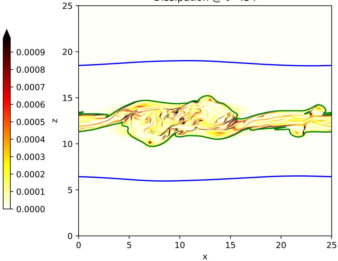
Dissipation @ t=454
