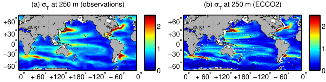
FIG. 2. Standard deviation of temperature ( \sigma_T ; °C) at 250 m (a) from observations in Forget and Wunsch (2007) and (b) from the ECCO2 state estimate. Seasonal variability is omitted in the standard deviation calculation.
