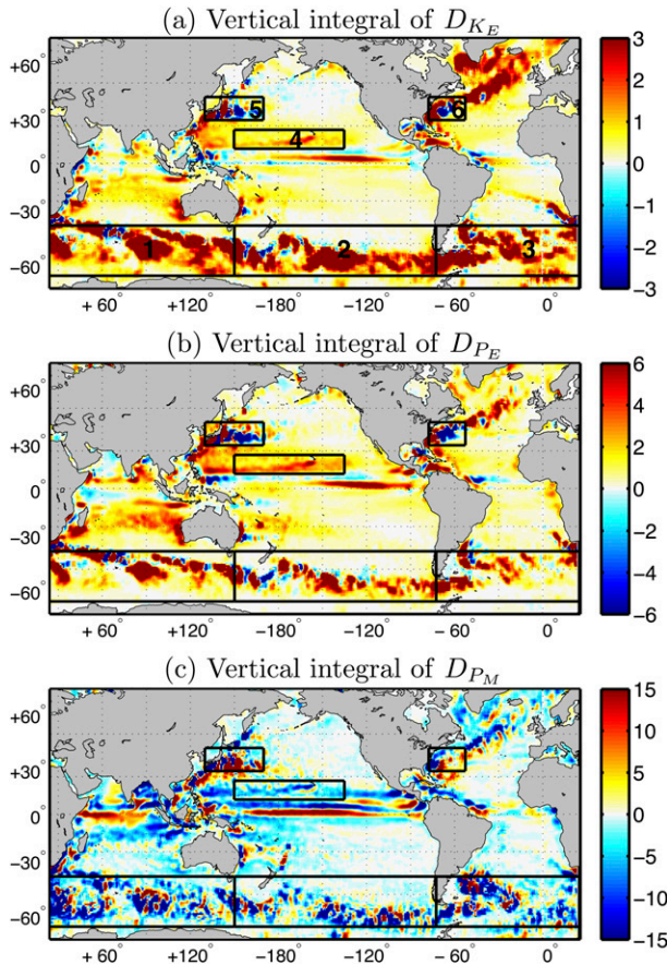
FIG. 5. The 3^\circ running-averaged (a) D_{K_E} , (b) D_{P_E} , and (c) D_{P_M} integrated over the whole water column ( 10^{-3} \text{ W m}^{-2} ). These terms describe energy change rates due to eddy-mean flow interaction through eddy density fluxes (Table 1). Positive (negative) D_{P_E} ( D_{P_M} ) means eddies (mean flow) gain (releases) potential energy through this process. Positive D_{K_E} means EAPE is converted to EKE. Magnitudes in the six black boxes are large. Energy routes in regions indicated by the six boxes are discussed in section 4b.
