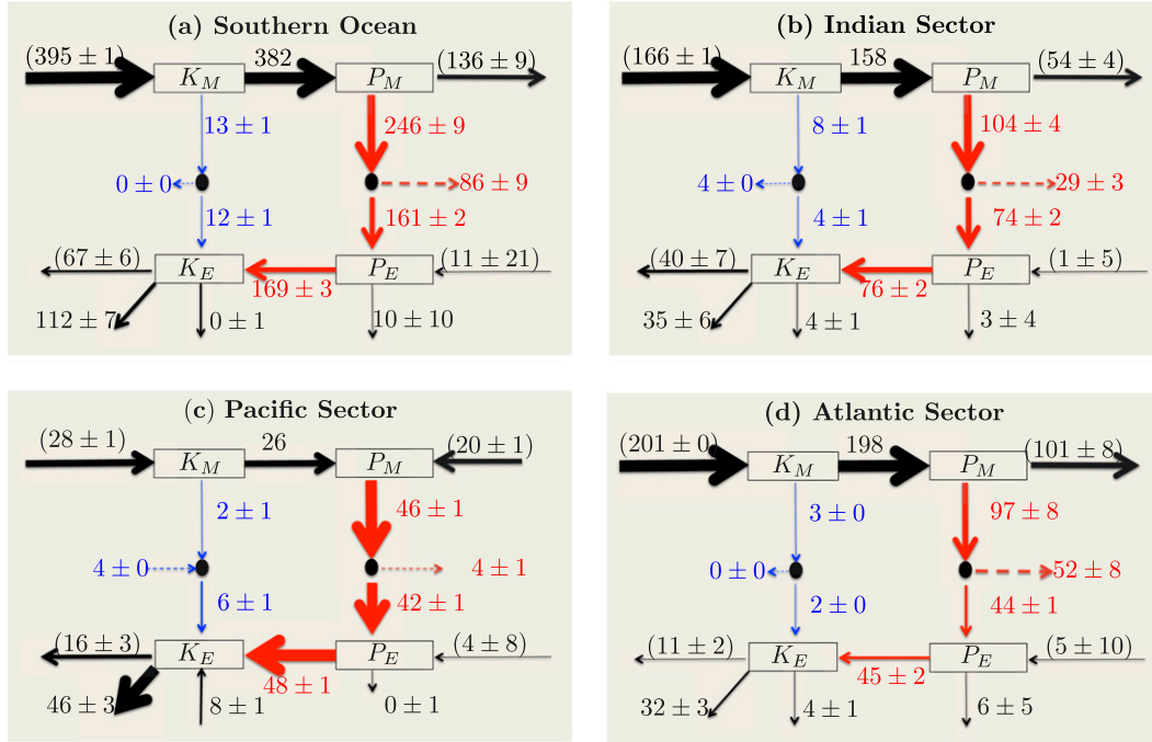
FIG. 7. The energy diagram in 10^9 W (GW) (Fig. 1) in the (a) whole Southern Ocean, (b) the Indian sector, (c) the Pacific sector, and (d) the Atlantic sector. These three sectors are, respectively, region 1, region 2, and region 3 in Fig. 5a. The whole Southern Ocean here denotes the sum of the three sectors. The contribution of the M terms to eddy growth is negligible. In the Indian and Atlantic sectors, only part of the energy released from MAPE through eddy–mean flow interaction supports the eddy energy growth in the same domain. In the Pacific sector, roughly all the MAPE released supports eddy energy growth in the same domain. Errors shown here are one standard error, as that in Table 2. We obtain the numbers in brackets from the residuals. These residuals also include the contribution of high-frequency motions to other terms in the energy budgets, since we use 3-day-averaged fields. Note that the time mean of the temporal change rate term is either zero or negligible and is not presented here. The imbalances, if they exist, are from the time mean of the temporal change rate term and the roundoff errors.
